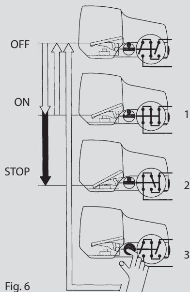
Fig. 6 Description of safety function on foot switches with mechanical lock
