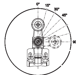
Adjustable lever
