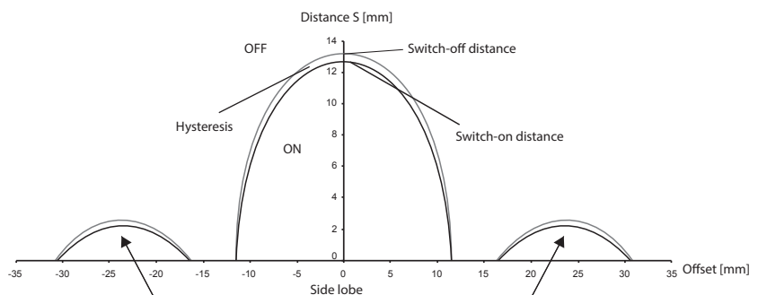
Metal can influence the sensing distance.
